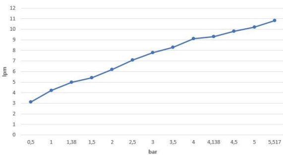
Flow Rate Chart
